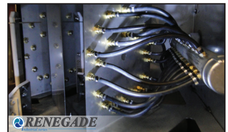
Strategically-placed wash nozzles deliver precision cleaning for custom fixtures.
