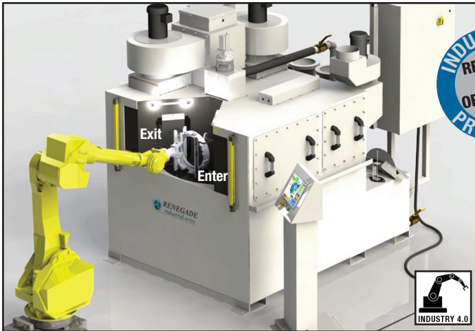
Renegade I-Series RTO Parts Washer (Shown with Optional Robotic Interface). Precision Cleaning and Drying in a Compact Footprint to Boost Cellular Operations. Dimensions: Length: 65-1/2"; Height: 91" inches; Width: 72-1/2" inches.
