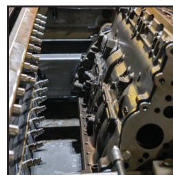
Rotary Fixture Assembly with Spray Manifold
