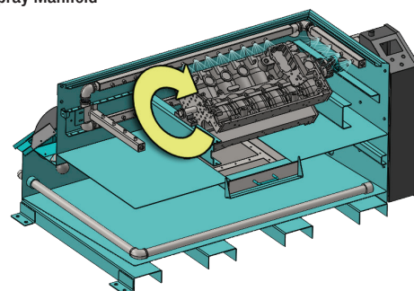
Rotary Fixture Assembly with Spray Manifold
