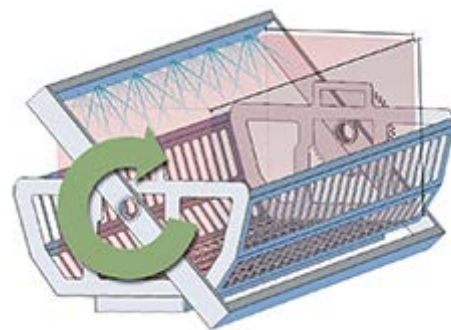
Interior Basket Assembly with Oscillating Spray Manifold
