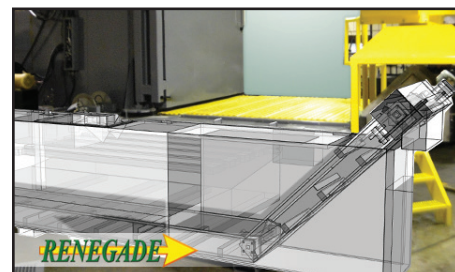
Sludge Conveyor for Heavy-Duty Grease Control
